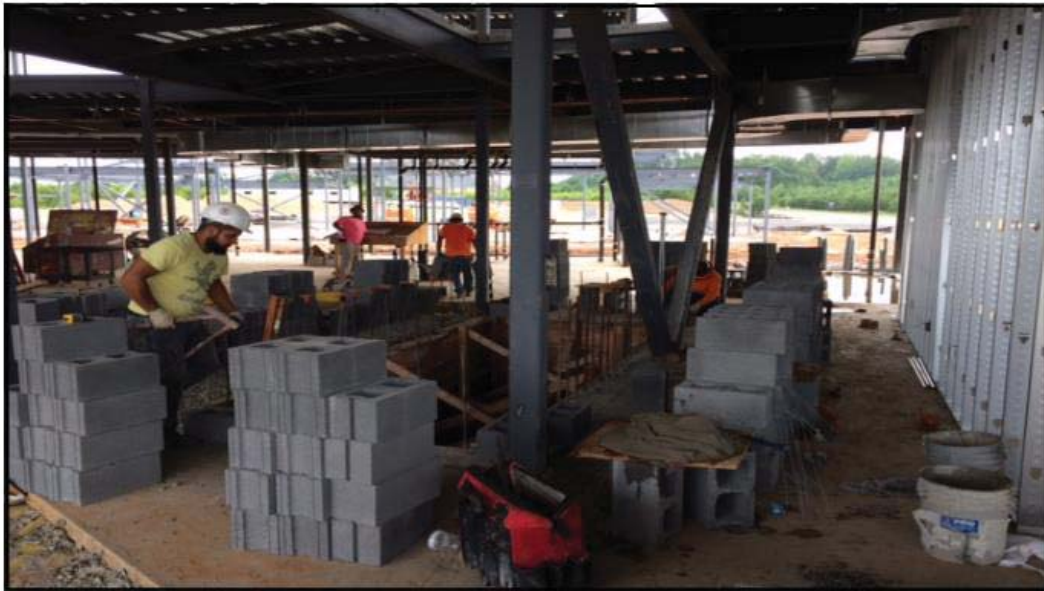
Block for Elevator
